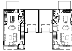
DUPLEX CONFIGURATION
